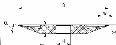
4BT9 D*T*X*W*H
