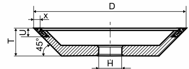
12V9-45° D*U*X*T*H
