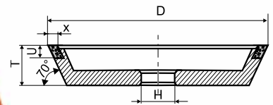
11V9-70° D*U*X*T*H
