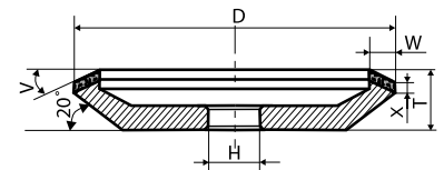
12V5-20 D*T*W*X*V*H
